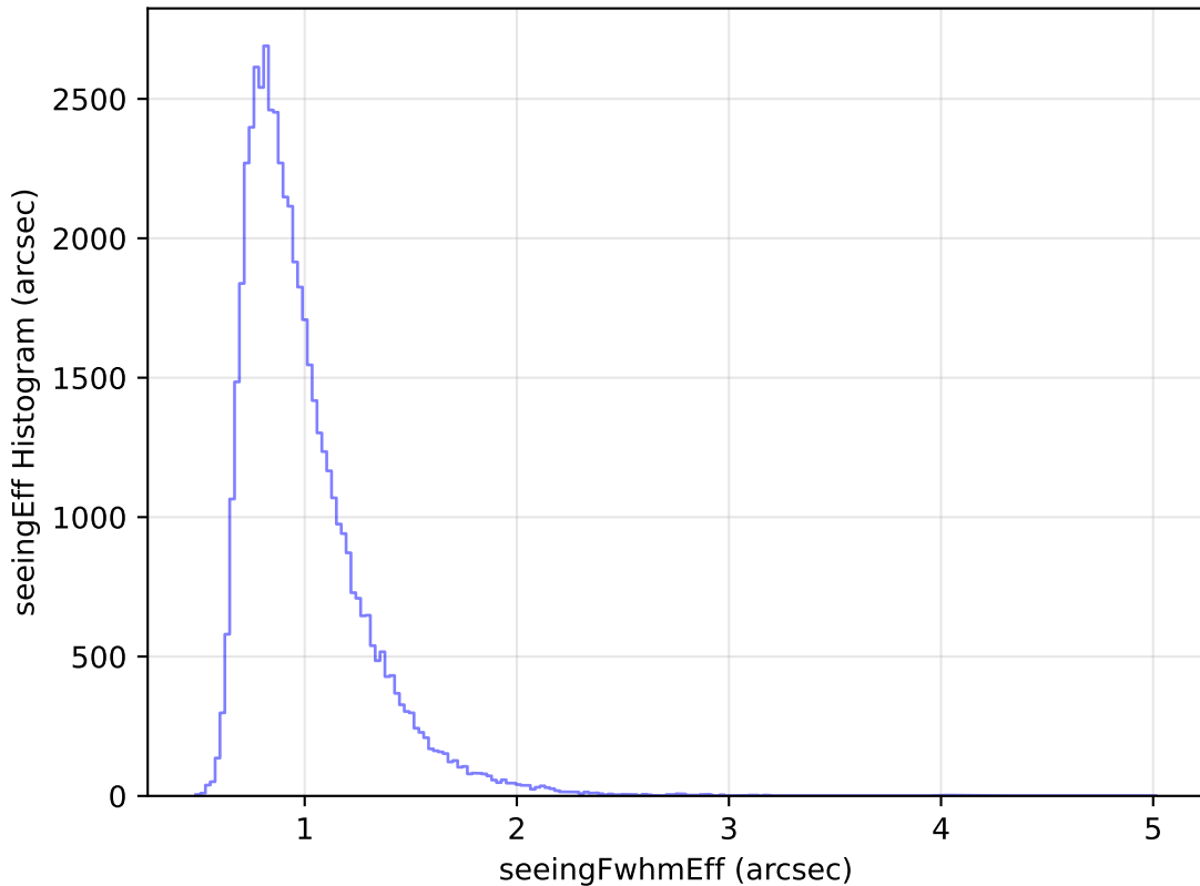
internal_u_expt38_nscale1.0v3.4_10yrs Yr 1 i band: seeingEff Histogram
