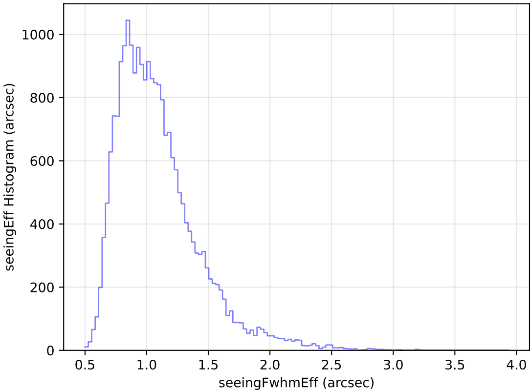
internal_u_expt38_nscale1.0v3.4_10yrs Yr 1 g band: seeingEff Histogram
