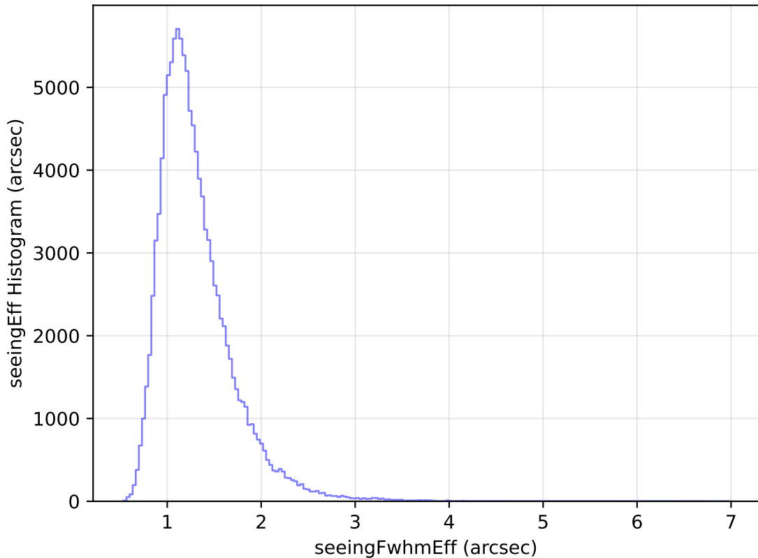
internal_u_expt38_nscale1.0v3.4_10yrs WFD u band: seeingEff Histogram
