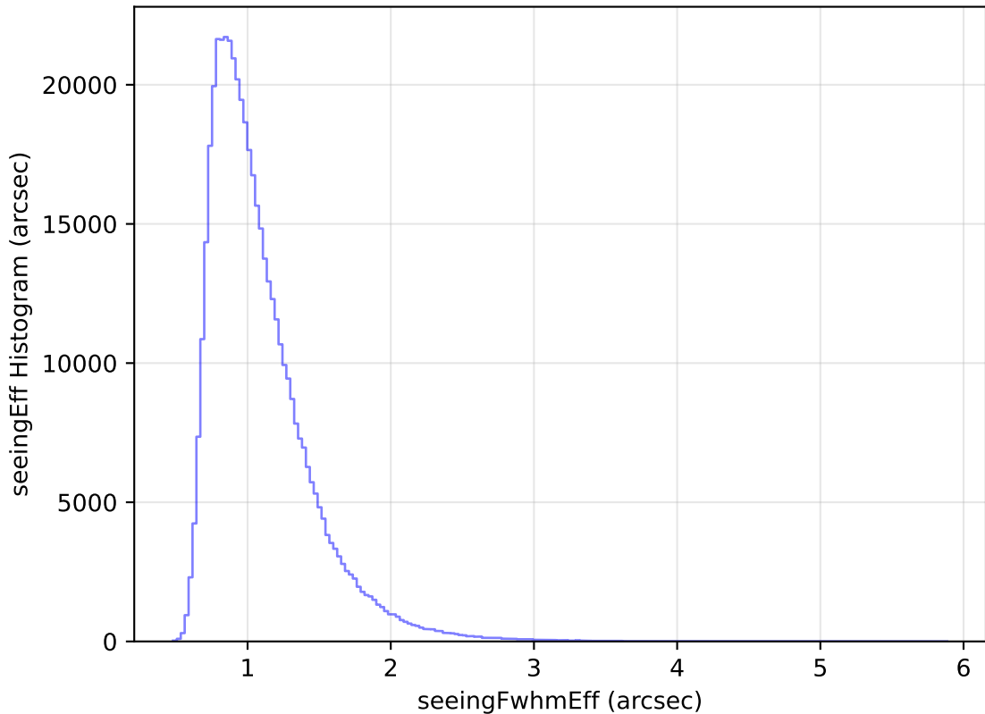
internal_u_expt38_nscale1.0v3.4_10yrs WFD i band: seeingEff Histogram
