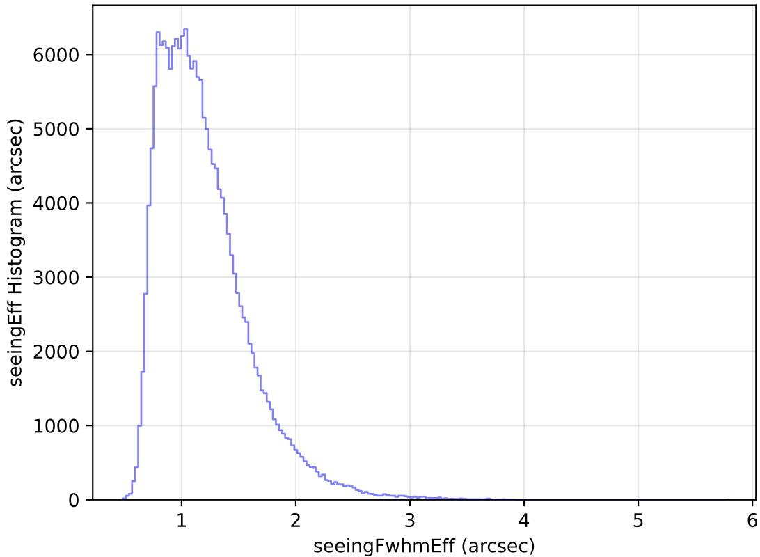
internal_u_expt38_nscale1.0v3.4_10yrs WFD g band: seeingEff Histogram
