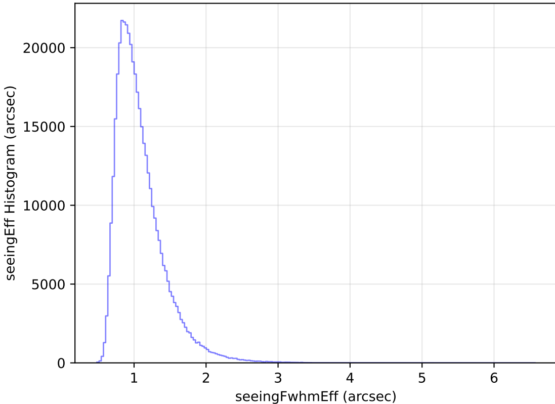
internal_u_expt38_nscale1.0v3.4_10yrs All sky z band: seeingEff Histogram
