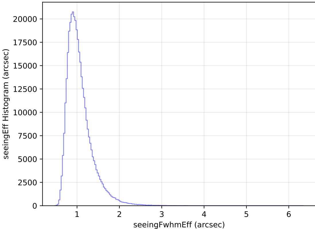
internal_u_expt38_nscale1.0v3.4_10yrs All sky y band: seeingEff Histogram
