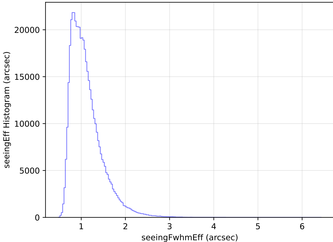
internal_u_expt38_nscale1.0v3.4_10yrs All sky r band: seeingEff Histogram
