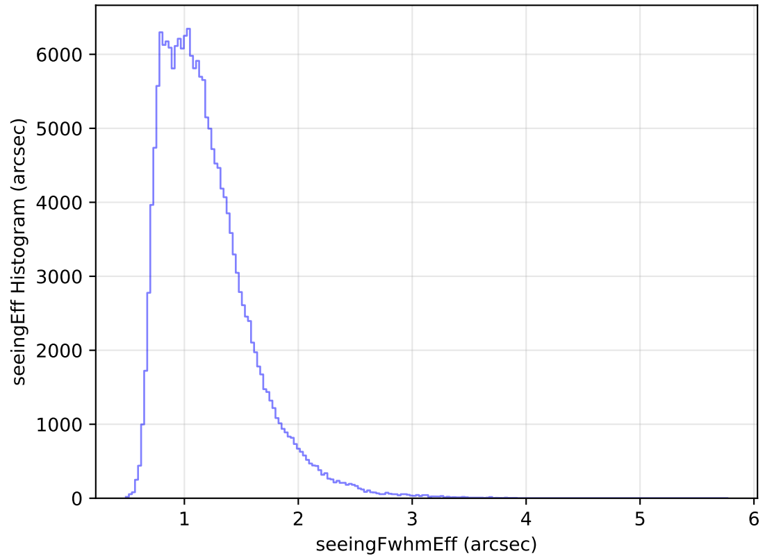
internal_u_expt38_nscale1.0v3.4_10yrs All sky g band: seeingEff Histogram
