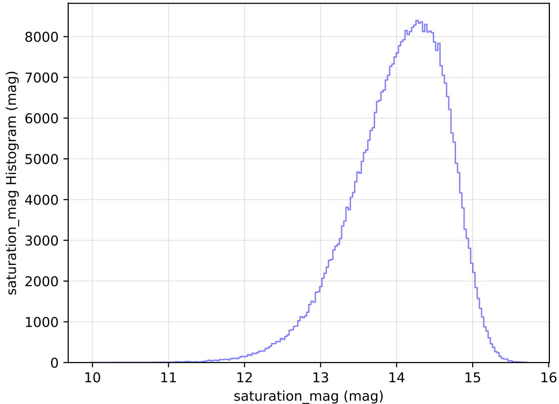
internal_u_expt38_nscale1.0v3.4_10yrs WFD z band: saturation_mag Histogram
