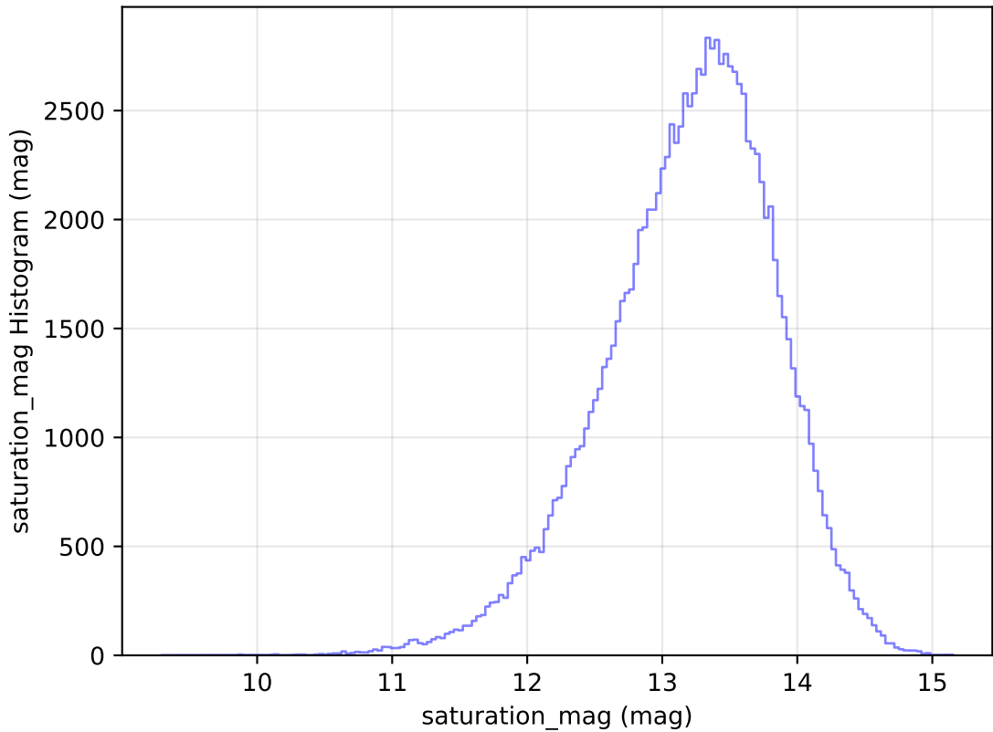
internal_u_expt38_nscale1.0v3.4_10yrs WFD u band: saturation_mag Histogram
