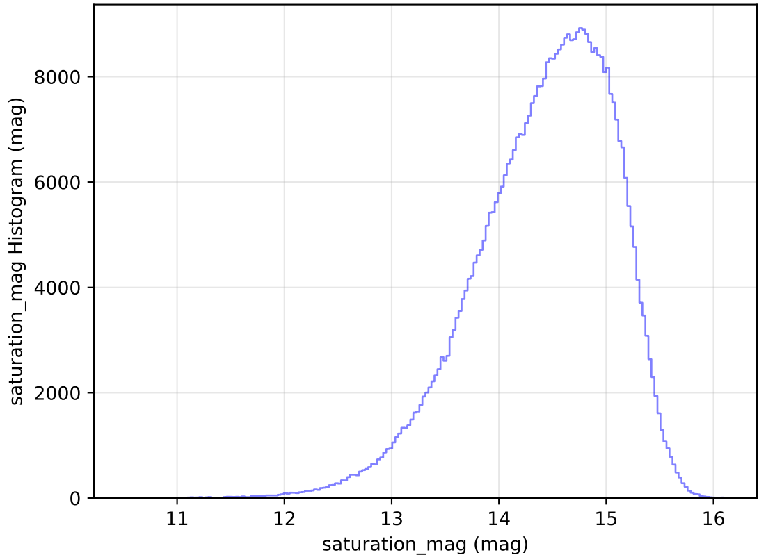
internal_u_expt38_nscale1.0v3.4_10yrs WFD i band: saturation_mag Histogram
