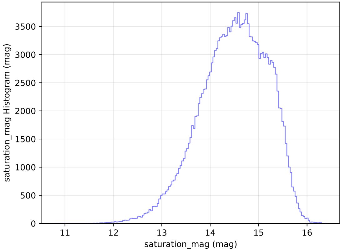
internal_u_expt38_nscale1.0v3.4_10yrs WFD g band: saturation_mag Histogram
