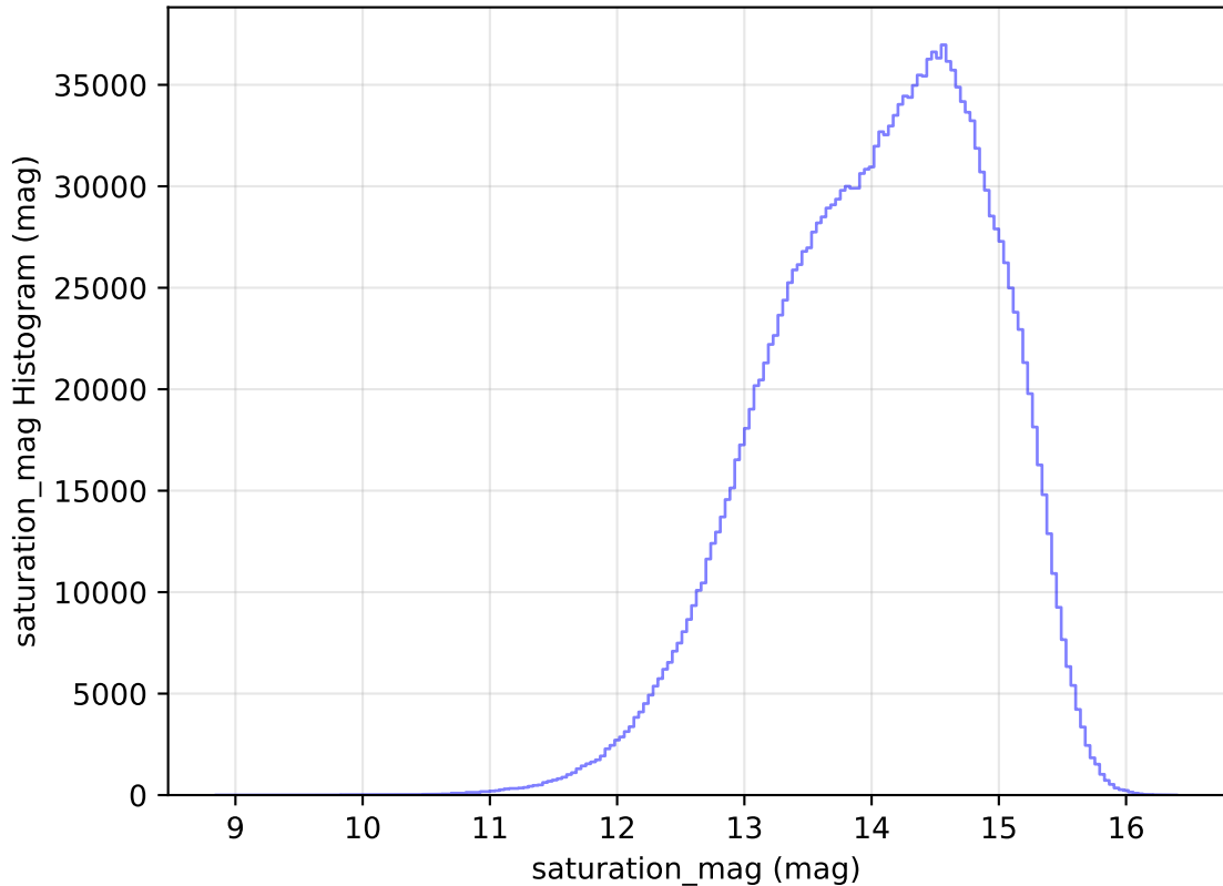
internal_u_expt38_nscale1.0v3.4_10yrs WFD all bands: saturation_mag Histogram
