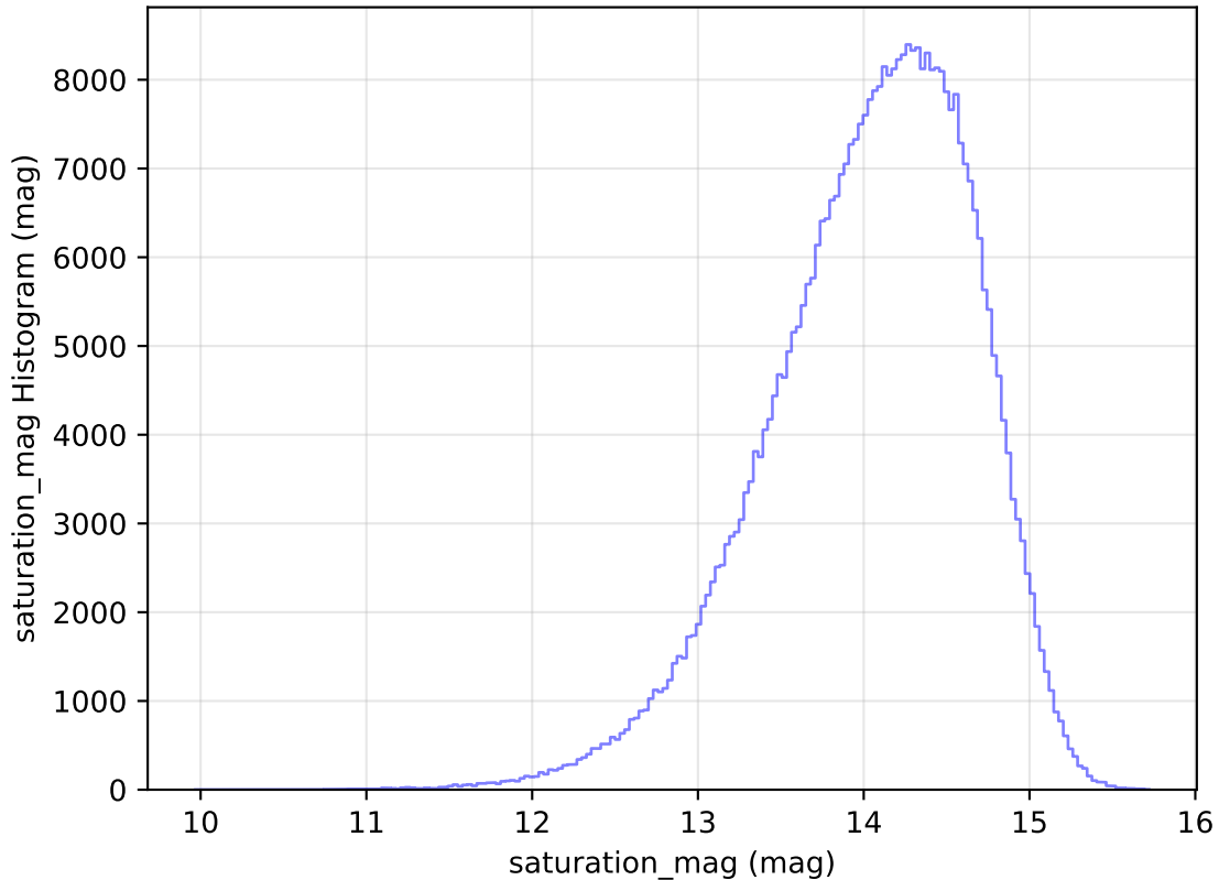
internal_u_expt38_nscale1.0v3.4_10yrs All sky z band: saturation_mag Histogram
