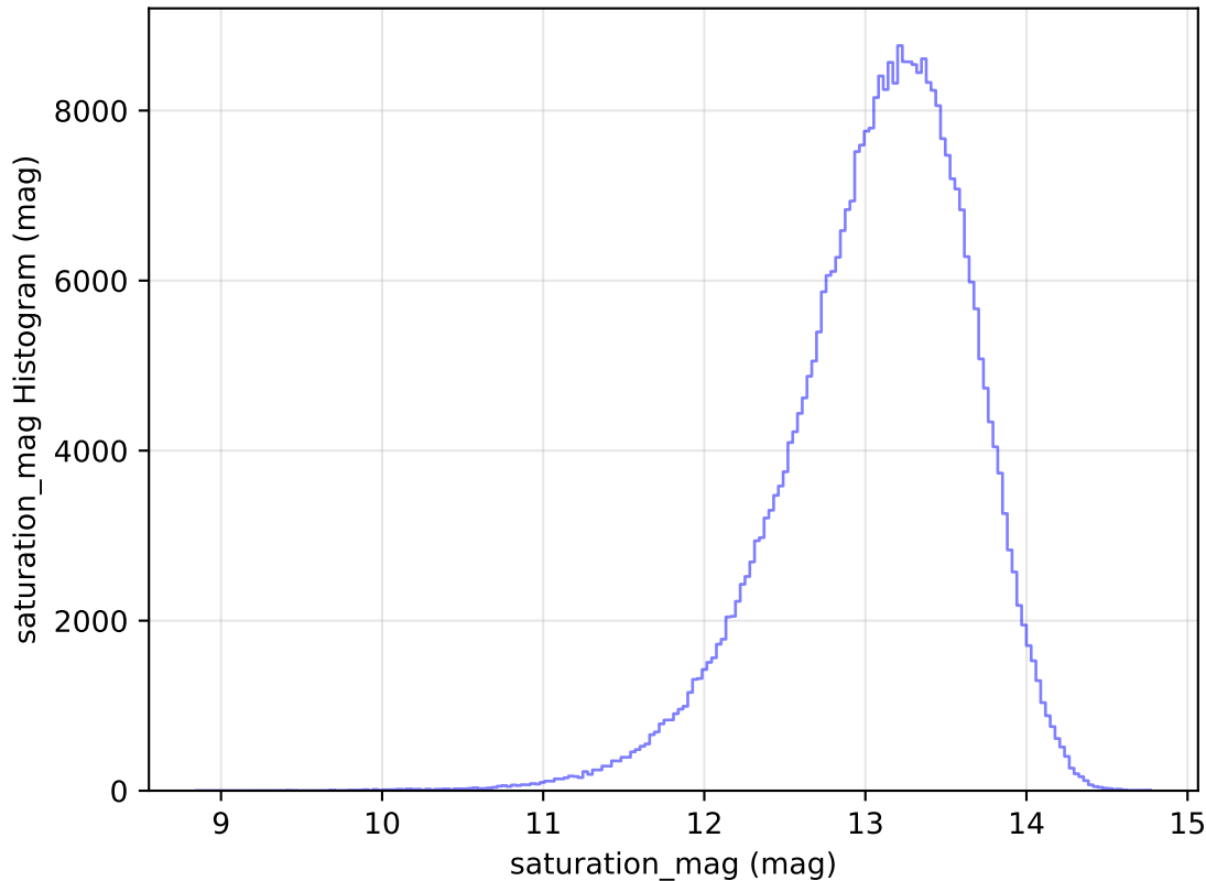
internal_u_expt38_nscale1.0v3.4_10yrs All sky y band: saturation_mag Histogram
