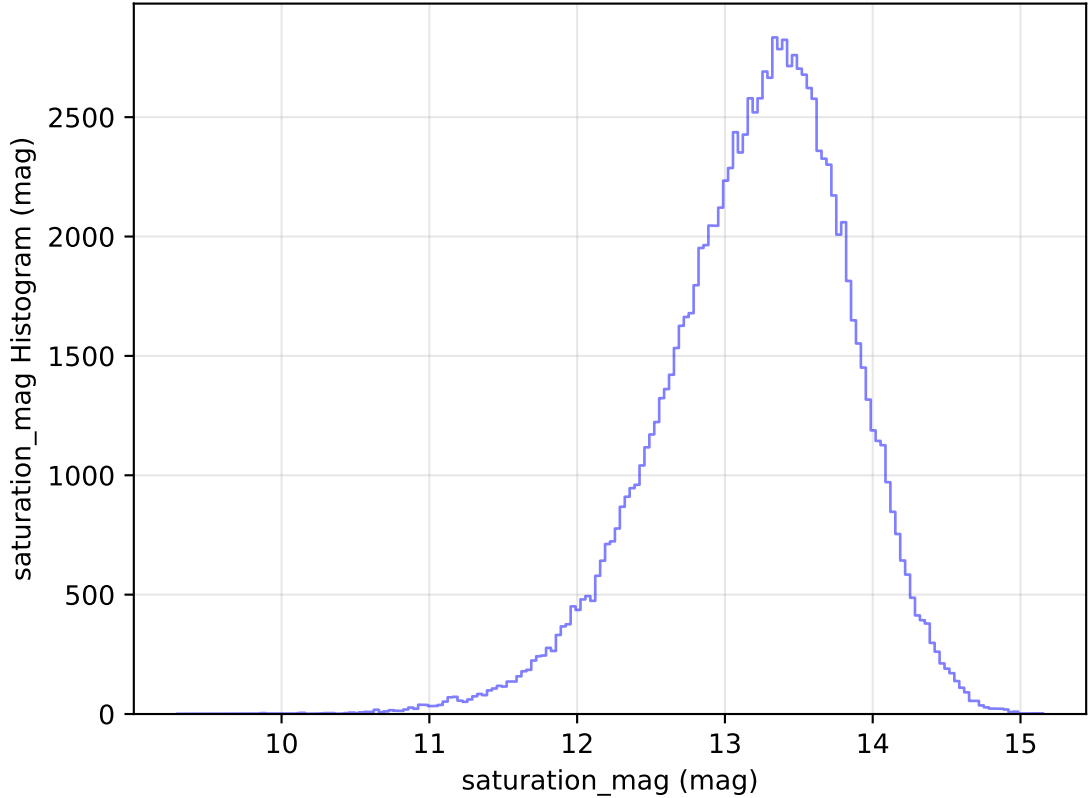
internal_u_expt38_nscale1.0v3.4_10yrs All sky u band: saturation_mag Histogram
