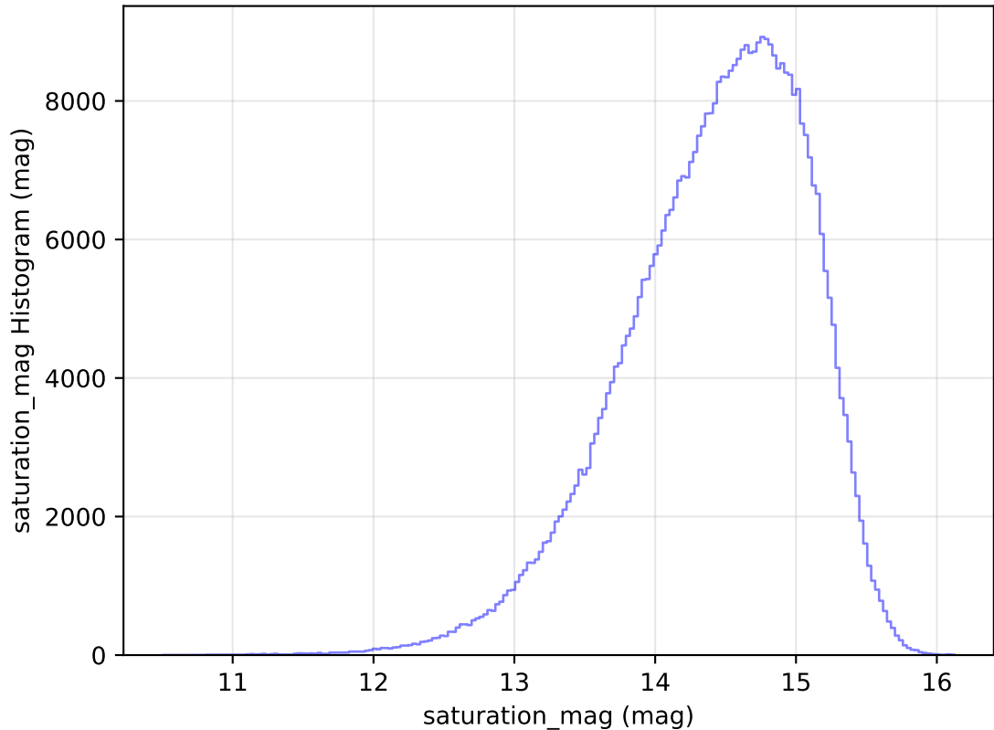
internal_u_expt38_nscale1.0v3.4_10yrs All sky i band: saturation_mag Histogram
