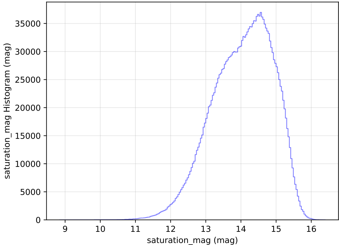
internal_u_expt38_nscale1.0v3.4_10yrs All sky all bands: saturation_mag Histogram
