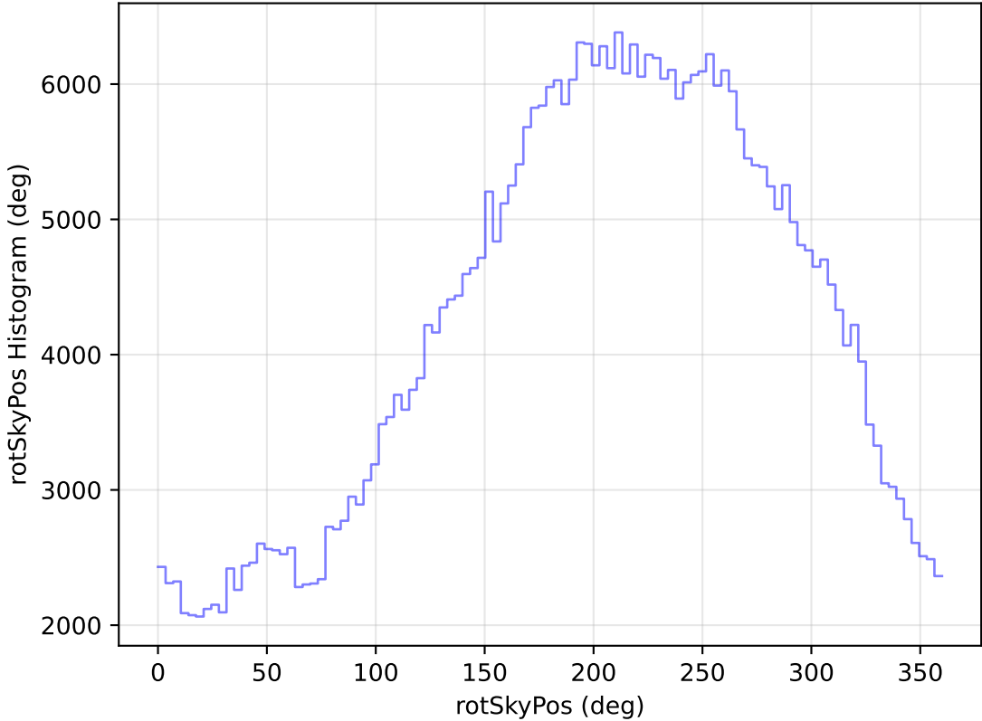
internal_u_expt38_nscale1.0v3.4_10yrs WFD z band: rotSkyPos Histogram
