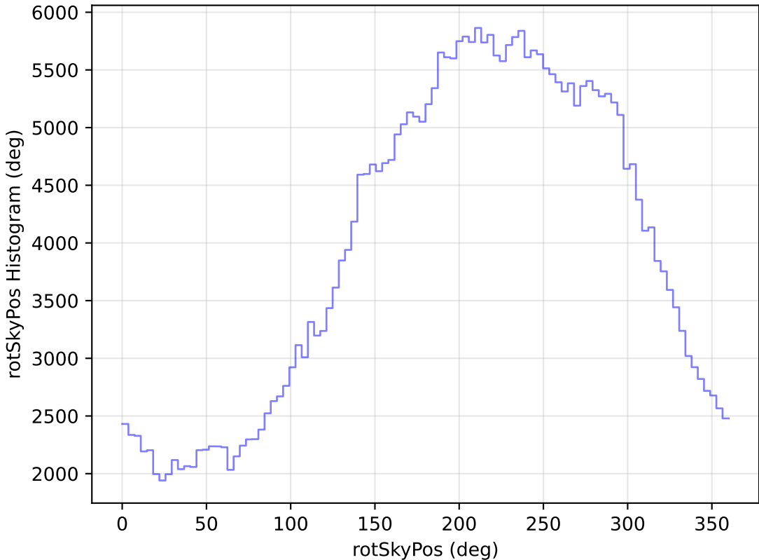
internal_u_expt38_nscale1.0v3.4_10yrs WFD y band: rotSkyPos Histogram
