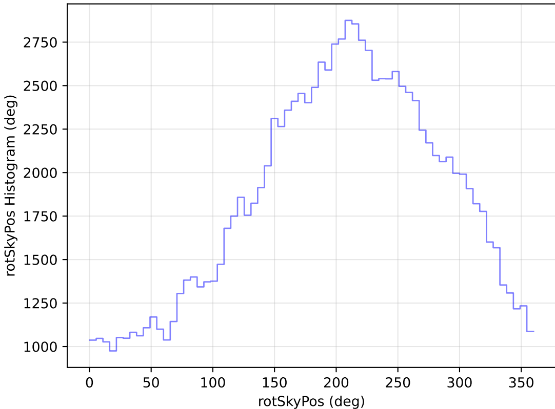
internal_u_expt38_nscale1.0v3.4_10yrs WFD u band: rotSkyPos Histogram
