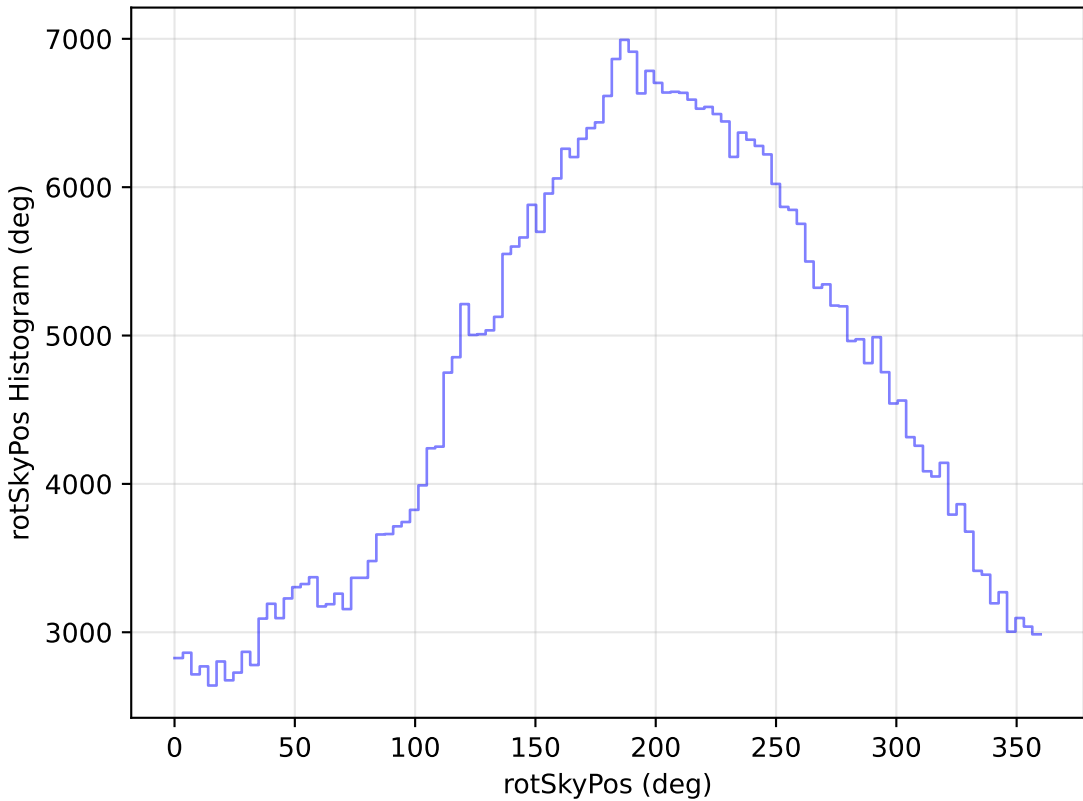
internal_u_expt38_nscale1.0v3.4_10yrs WFD r band: rotSkyPos Histogram
