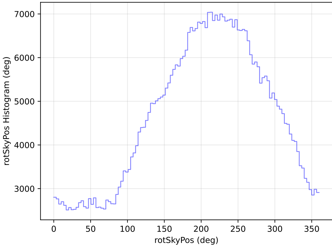
internal_u_expt38_nscale1.0v3.4_10yrs WFD i band: rotSkyPos Histogram
