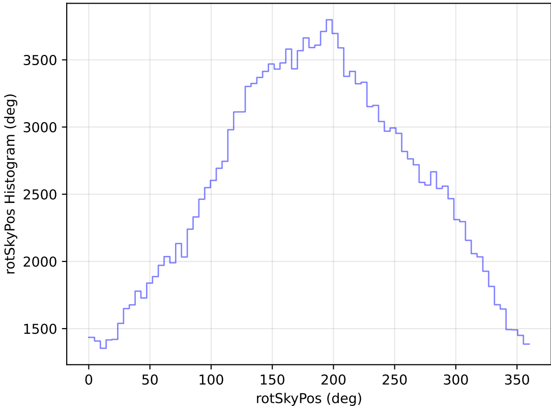
internal_u_expt38_nscale1.0v3.4_10yrs WFD g band: rotSkyPos Histogram
