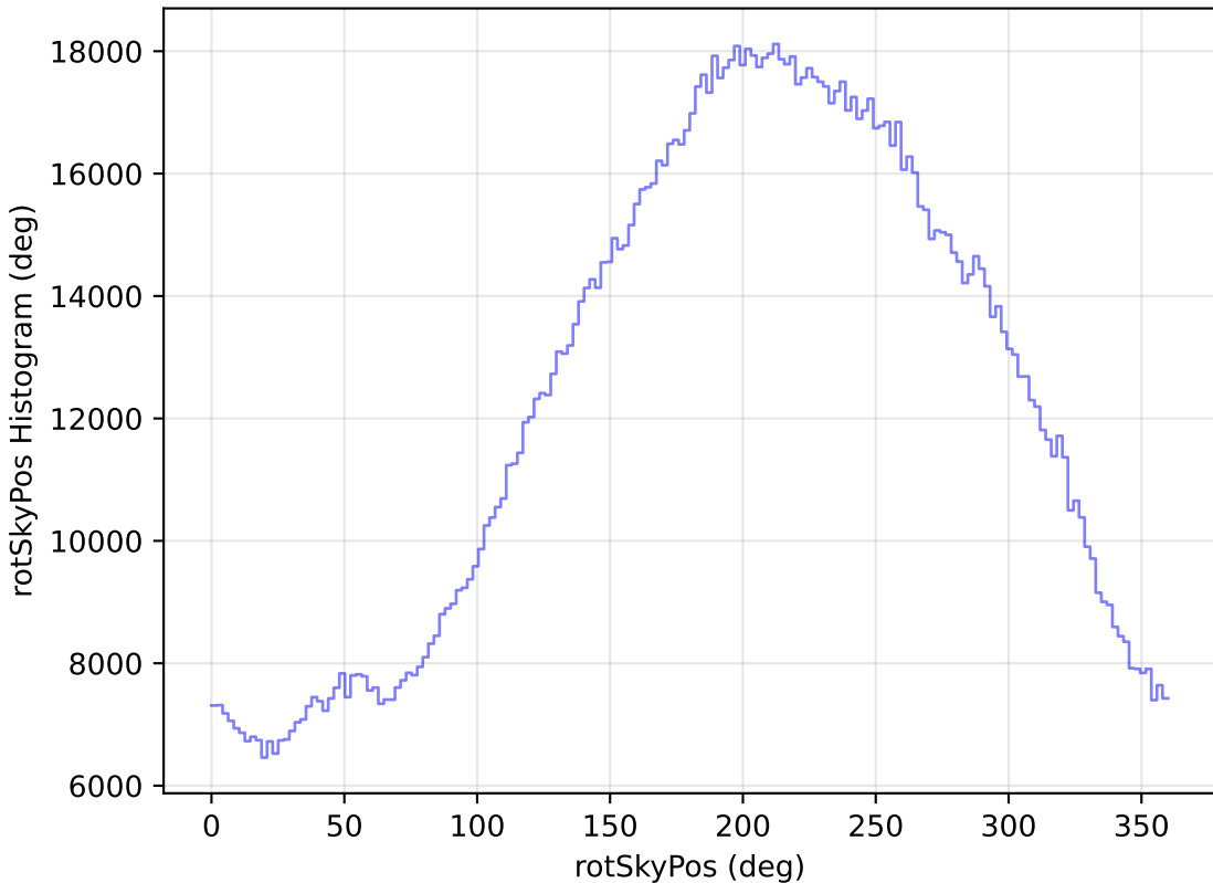
internal_u_expt38_nscale1.0v3.4_10yrs WFD all bands: rotSkyPos Histogram
