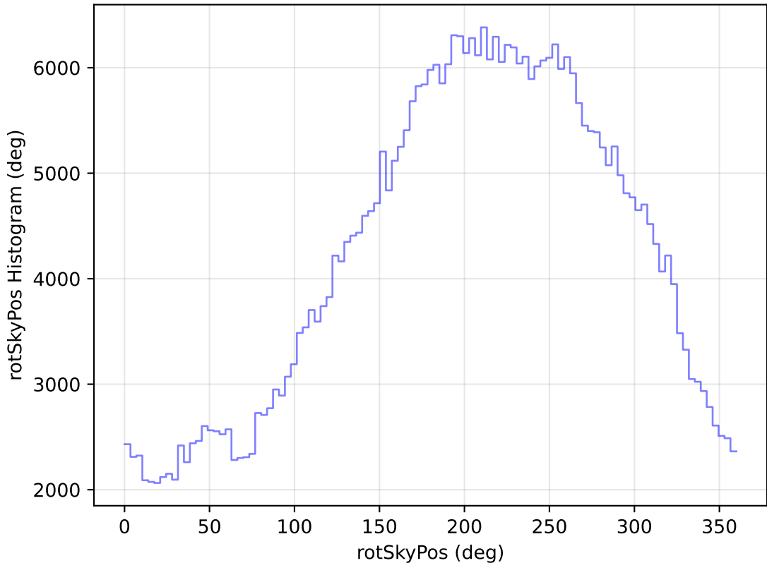
internal_u_expt38_nscale1.0v3.4_10yrs All sky z band: rotSkyPos Histogram
