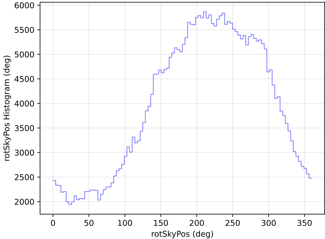
internal_u_expt38_nscale1.0v3.4_10yrs All sky y band: rotSkyPos Histogram
