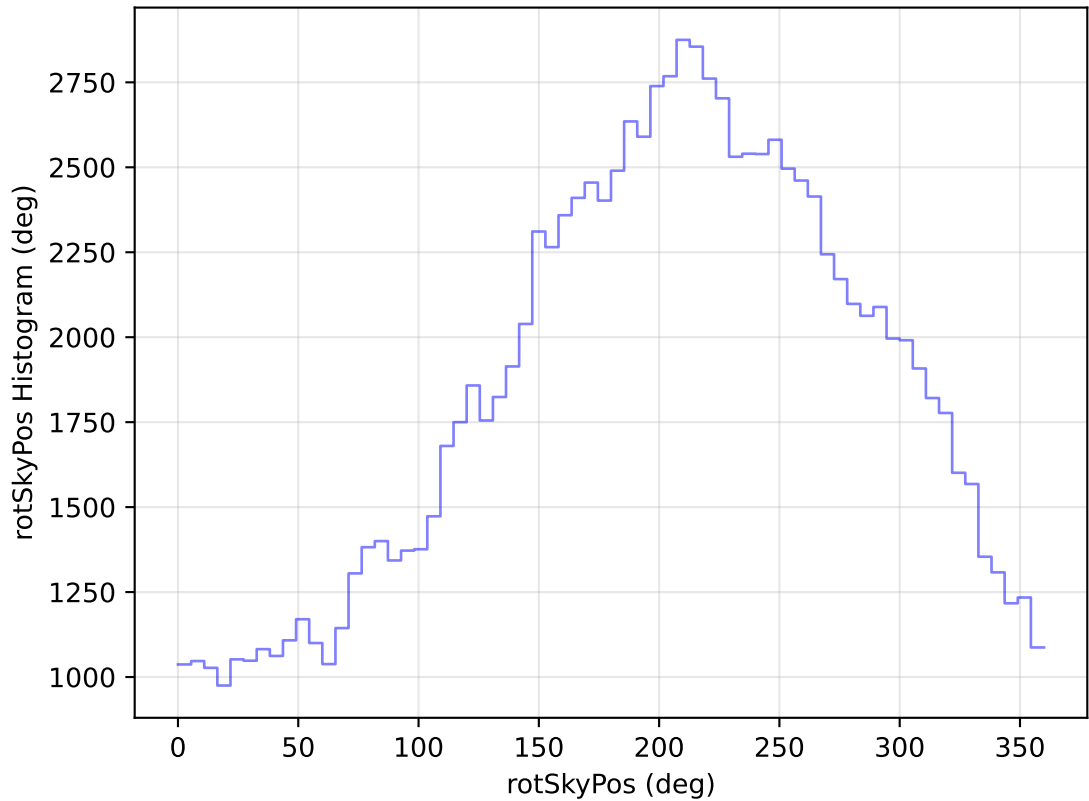
internal_u_expt38_nscale1.0v3.4_10yrs All sky u band: rotSkyPos Histogram
