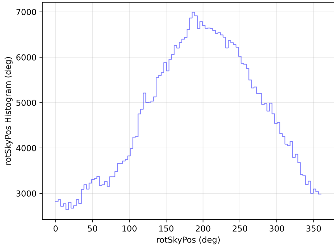
internal_u_expt38_nscale1.0v3.4_10yrs All sky r band: rotSkyPos Histogram
