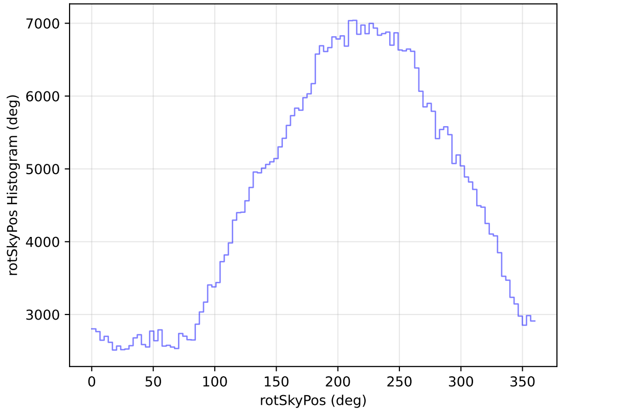
internal_u_expt38_nscale1.0v3.4_10yrs All sky i band: rotSkyPos Histogram
