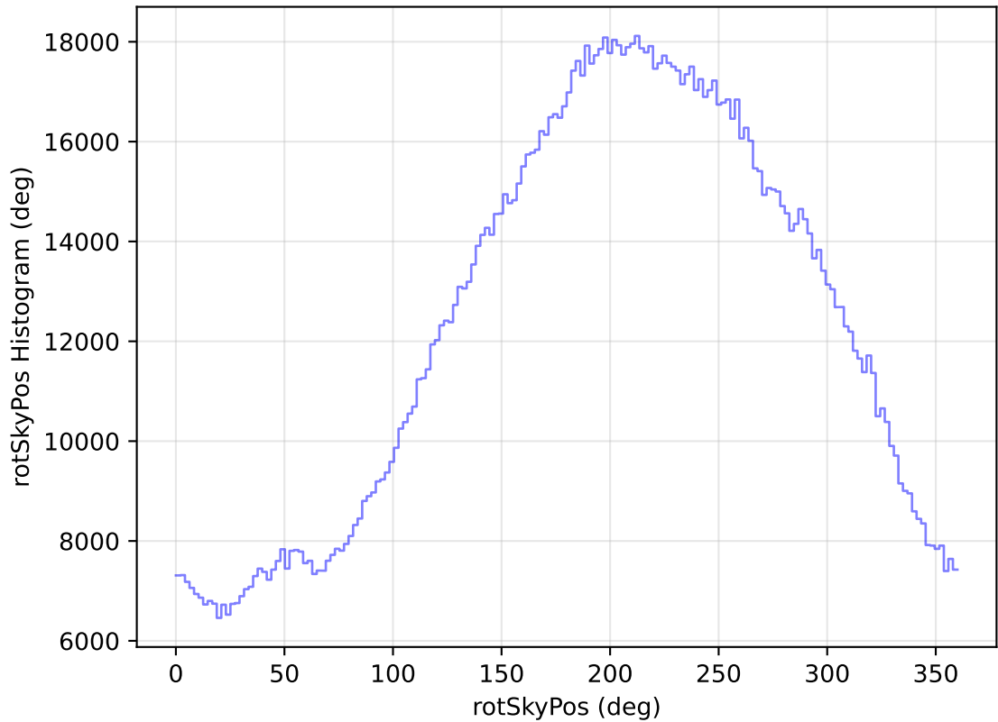
internal_u_expt38_nscale1.0v3.4_10yrs All sky all bands: rotSkyPos Histogram
