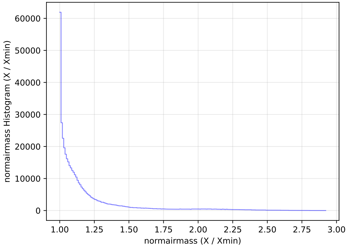
internal_u_expt38_nscale1.0v3.4_10yrs WFD z band: normairmass Histogram
