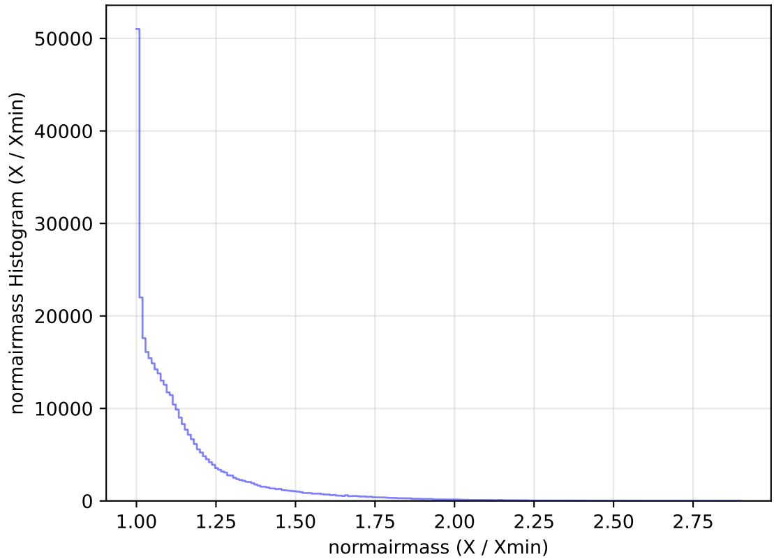
internal_u_expt38_nscale1.0v3.4_10yrs WFD y band: normairmass Histogram
