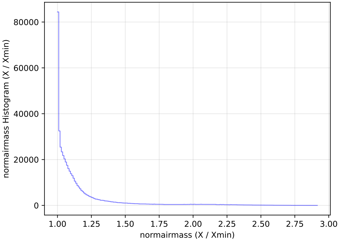
internal_u_expt38_nscale1.0v3.4_10yrs WFD i band: normairmass Histogram
