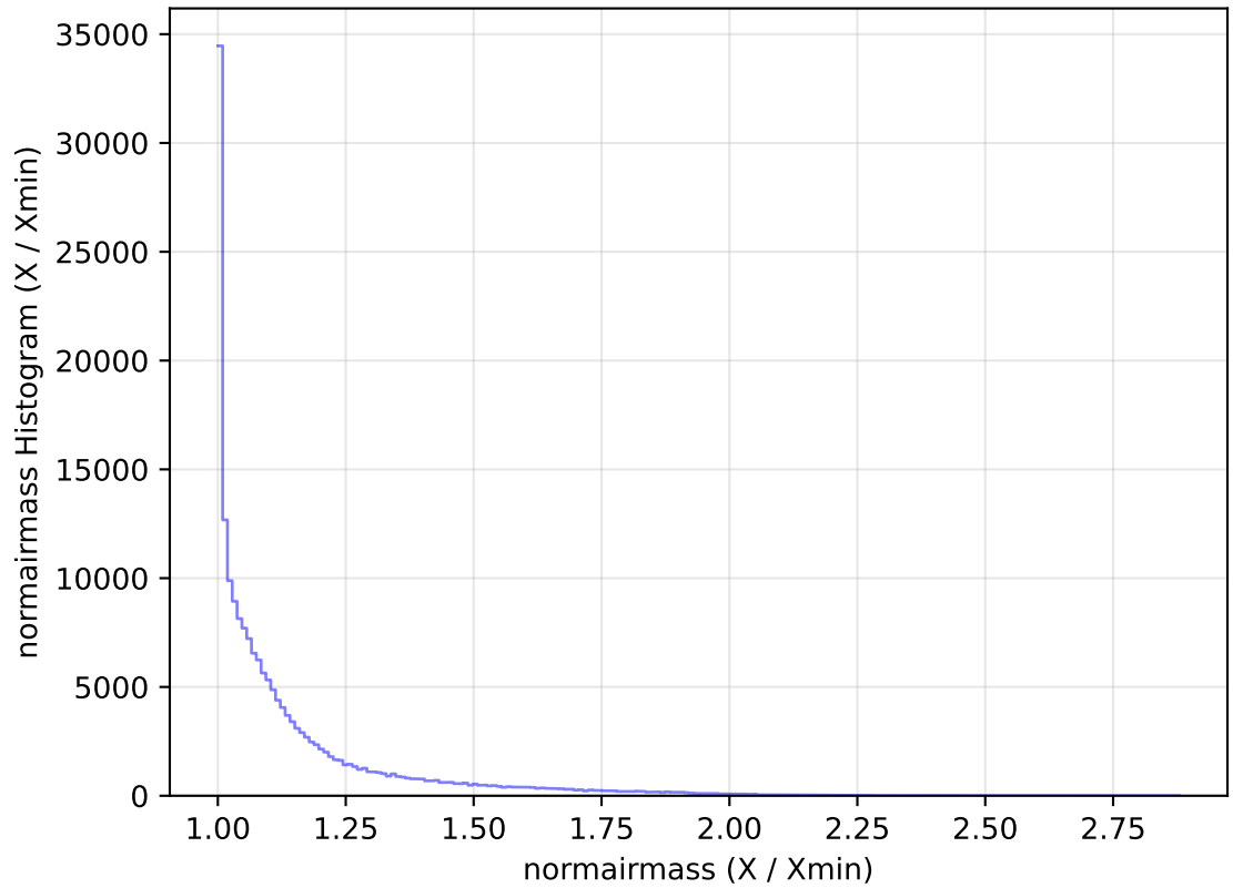
internal_u_expt38_nscale1.0v3.4_10yrs WFD g band: normairmass Histogram
