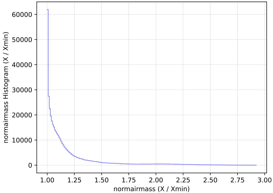
internal_u_expt38_nscale1.0v3.4_10yrs All sky z band: normairmass Histogram
