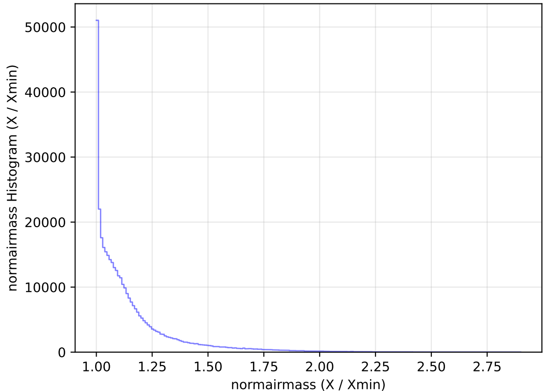
internal_u_expt38_nscale1.0v3.4_10yrs All sky y band: normairmass Histogram
