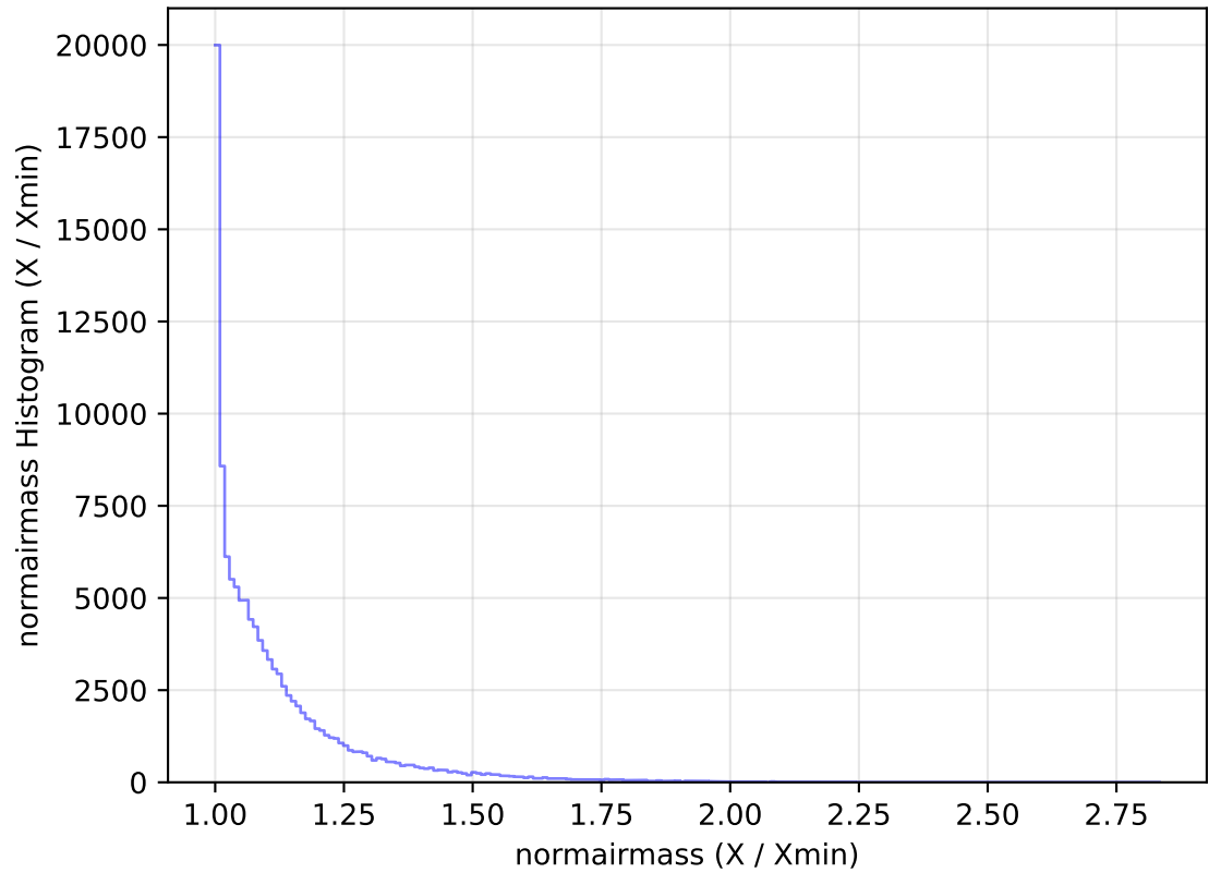
internal_u_expt38_nscale1.0v3.4_10yrs All sky u band: normairmass Histogram
