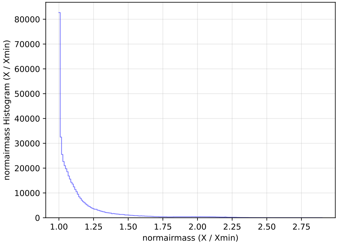
internal_u_expt38_nscale1.0v3.4_10yrs All sky r band: normairmass Histogram
