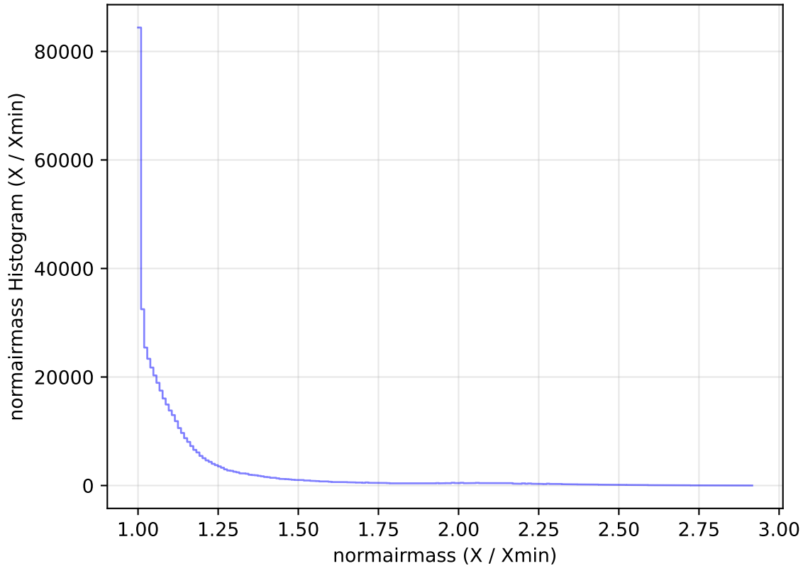
internal_u_expt38_nscale1.0v3.4_10yrs All sky i band: normairmass Histogram
