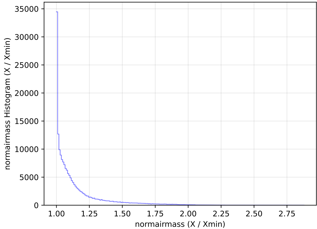
internal_u_expt38_nscale1.0v3.4_10yrs All sky g band: normairmass Histogram
