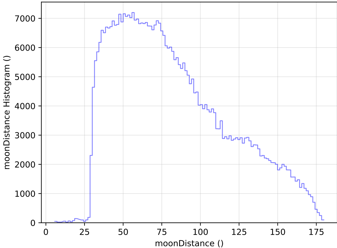
internal_u_expt38_nscale1.0v3.4_10yrs WFD z band: moonDistance Histogram
