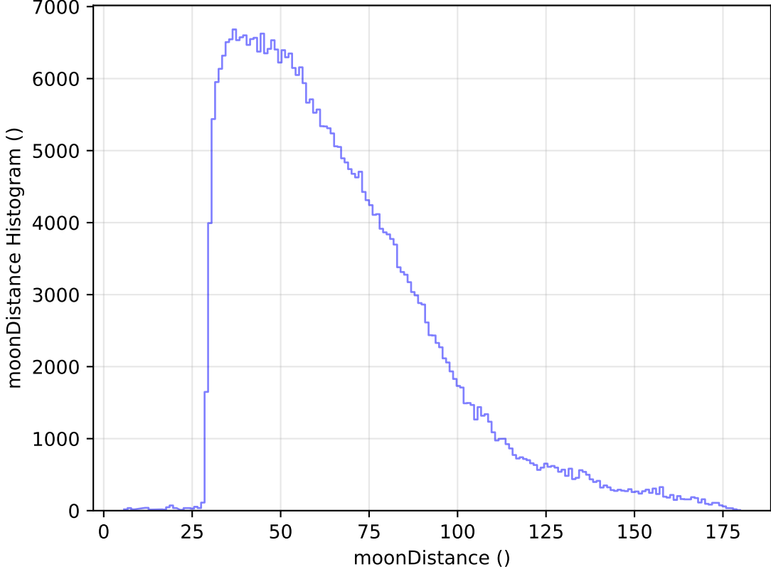
internal_u_expt38_nscale1.0v3.4_10yrs WFD y band: moonDistance Histogram
