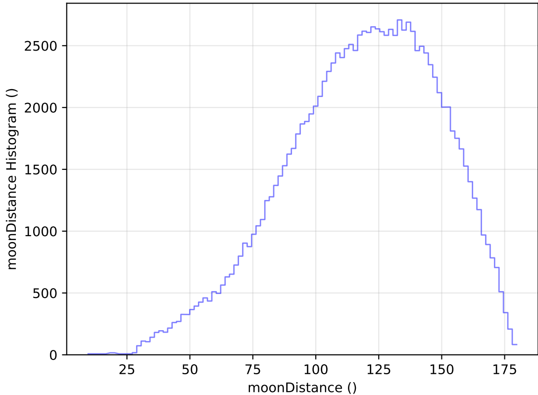
internal_u_expt38_nscale1.0v3.4_10yrs WFD u band: moonDistance Histogram
