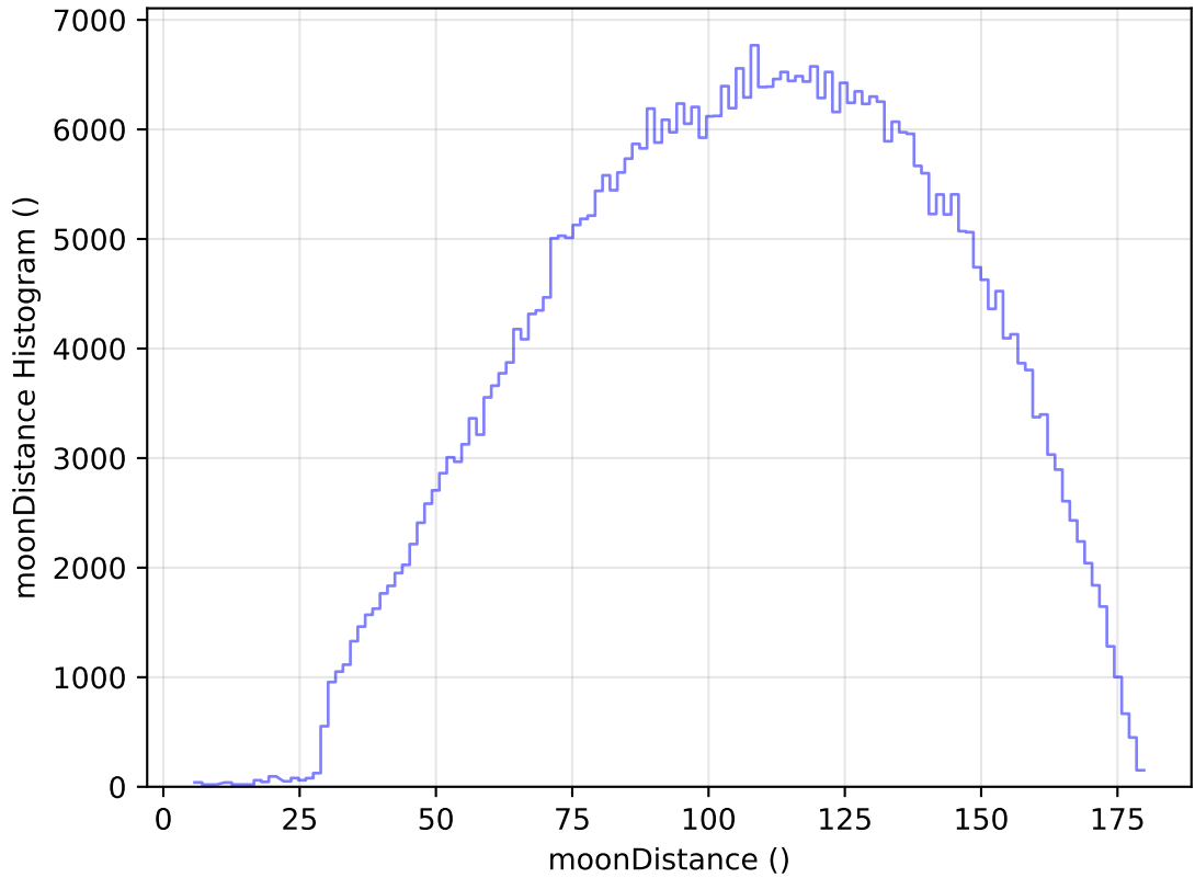
internal_u_expt38_nscale1.0v3.4_10yrs WFD r band: moonDistance Histogram
