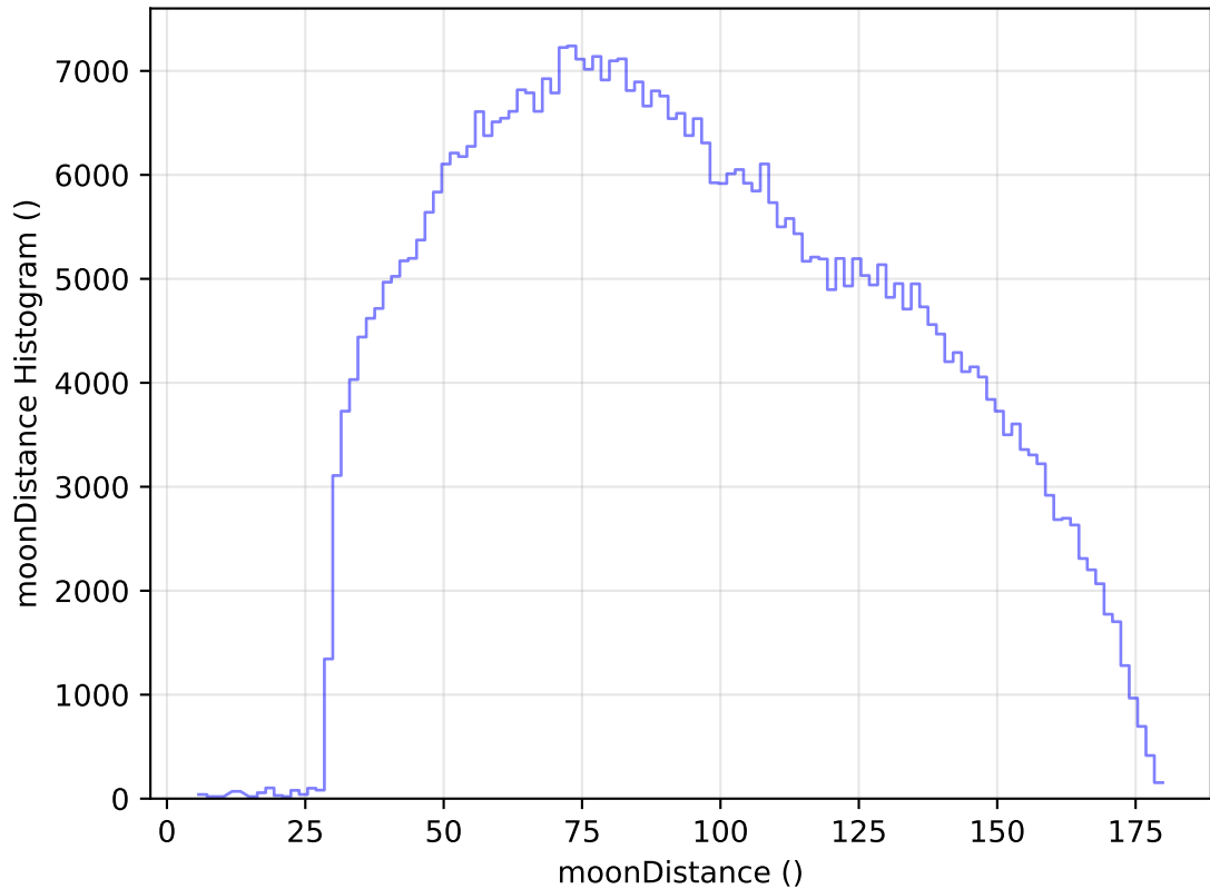
internal_u_expt38_nscale1.0v3.4_10yrs WFD i band: moonDistance Histogram
