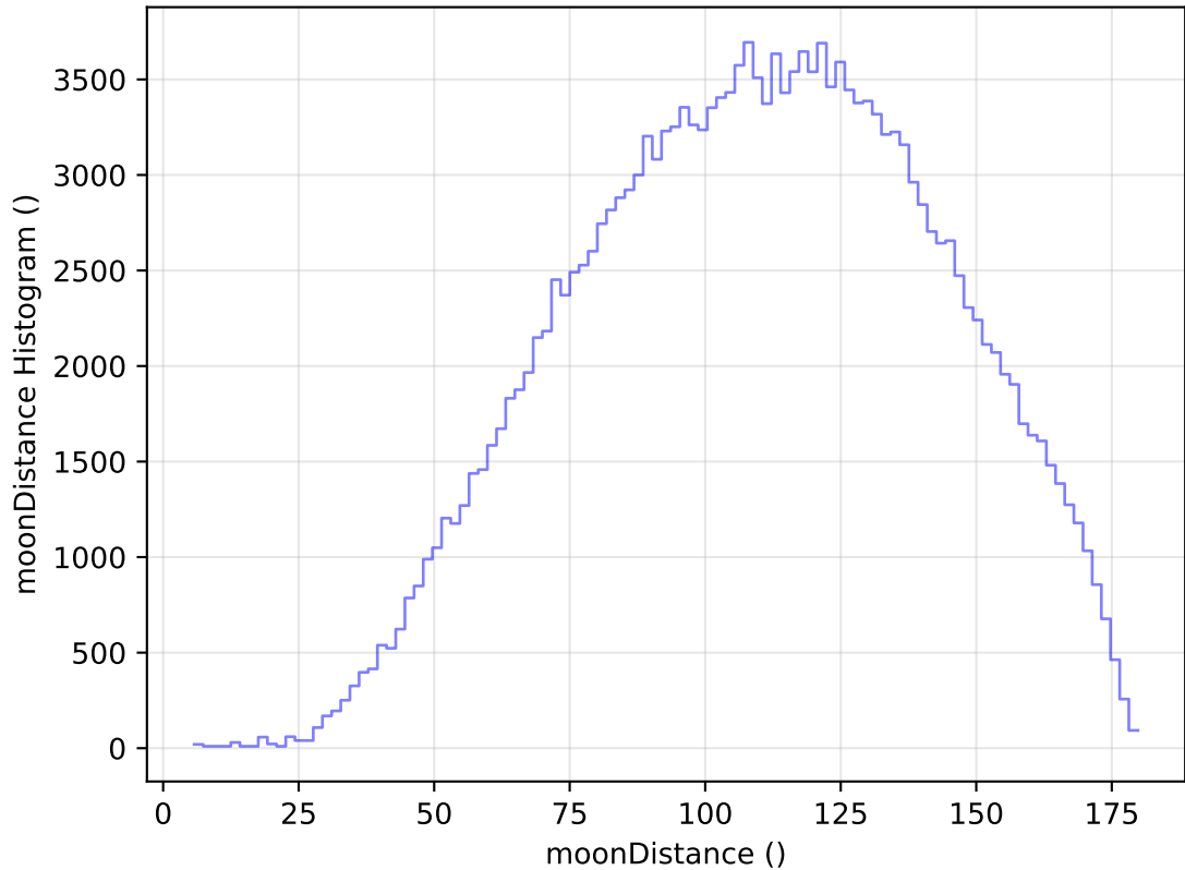
internal_u_expt38_nscale1.0v3.4_10yrs WFD g band: moonDistance Histogram
