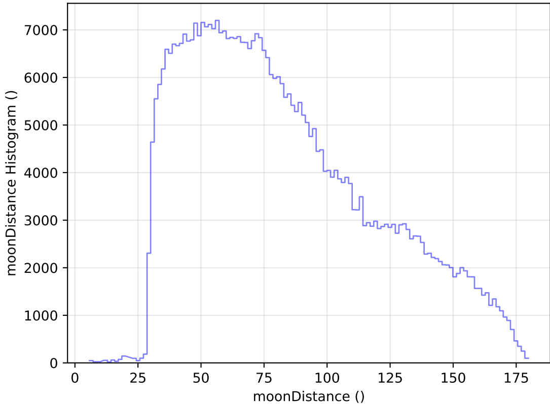
internal_u_expt38_nscale1.0v3.4_10yrs All sky z band: moonDistance Histogram
