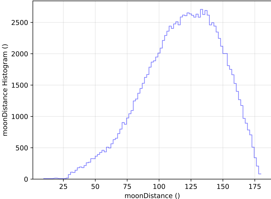
internal_u_expt38_nscale1.0v3.4_10yrs All sky u band: moonDistance Histogram
